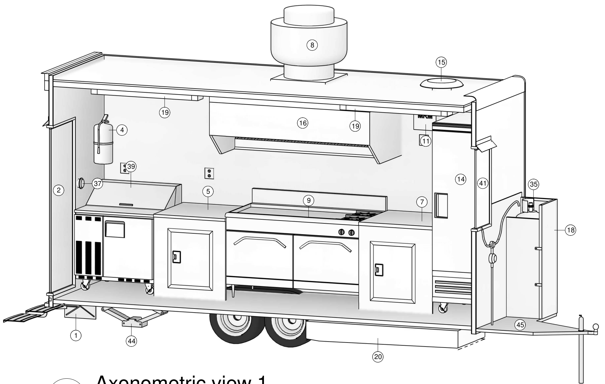
1 Axonometric view 1
